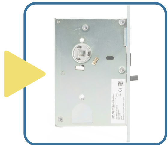
Manipulation protection on Mortise variant's lock case
